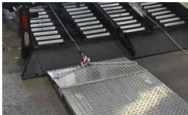
The trailer is equipped with scale rollers, winches and a hydraulic tilt package which virtually eliminate the need for manual labor when pulling the scale up the trailer.
