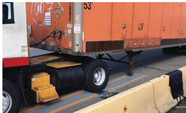
LS630-WIM™ Systems were chosen as an efficient method to screen incoming containers for proper gross weight to ensure safe transport.
