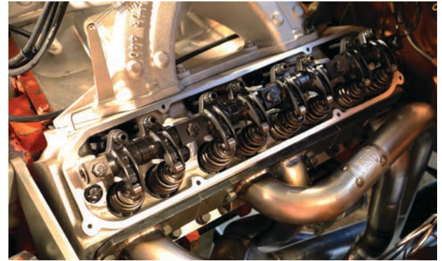
The chance of valve spring failure in high-performance engines can be reduced through a proper maintenance and testing program.
